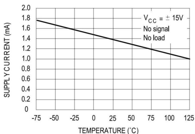
Fig 4. Supply Current vs. Ambient Temperature(per Channel)
