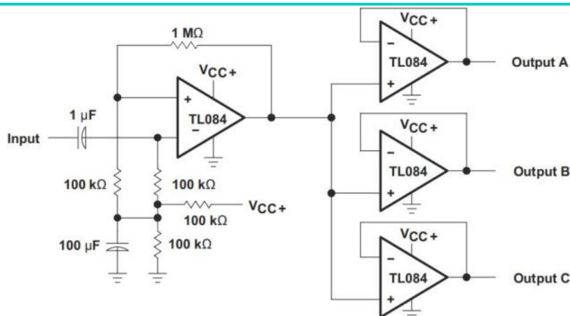
Figure 2. Audio Distribution Amplifier
