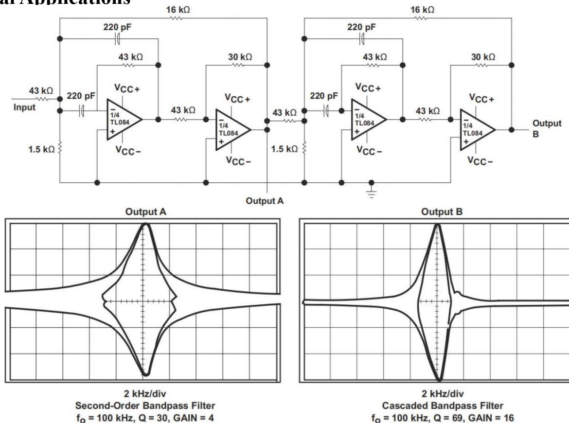
Figure 1. Positive Feedback Bandpass Filter
