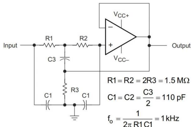
Figure 4. High Q Notch Filter
