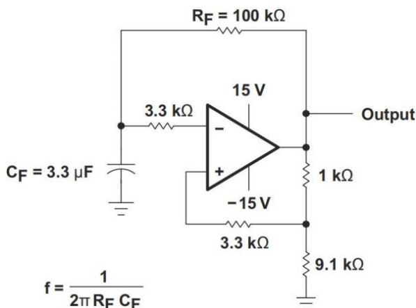
Figure 3. 0.5Hz Square Wave Oscillator
