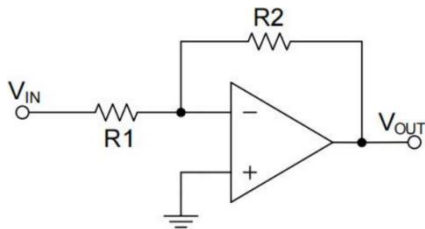
Figure 1. Inverting Amplifier
