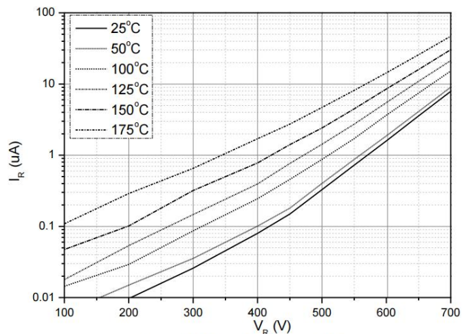
Figure 2. Reverse Characteristics
