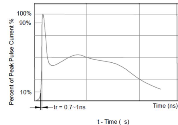
Fig2. Contact Discharge Current Waveform ( IEC 61000-4-2)
