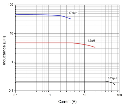
Inductance VS Current
