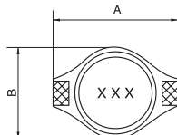
Fig.1 : Type D(No magnetic cover)
