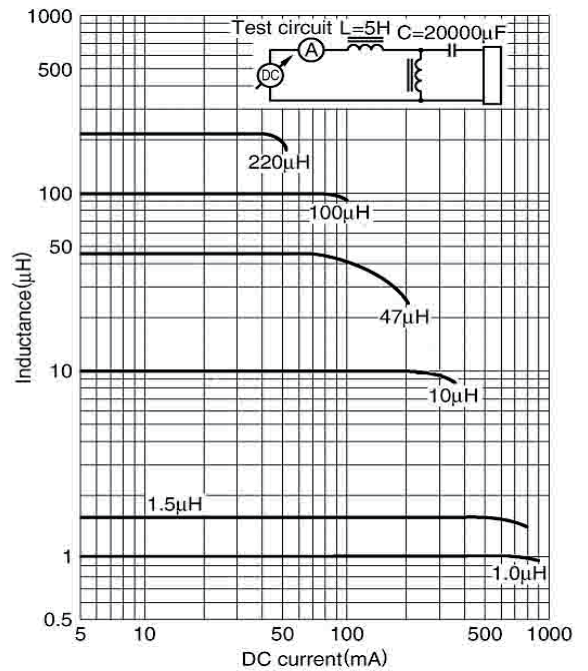
Inductance- DC current characteristic
