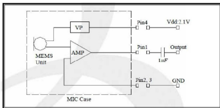
Measurement circuit
