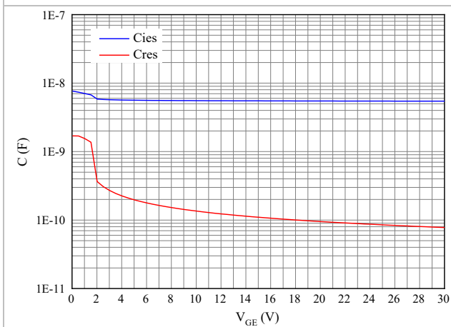
Figure 9. Capacitance characteristic
