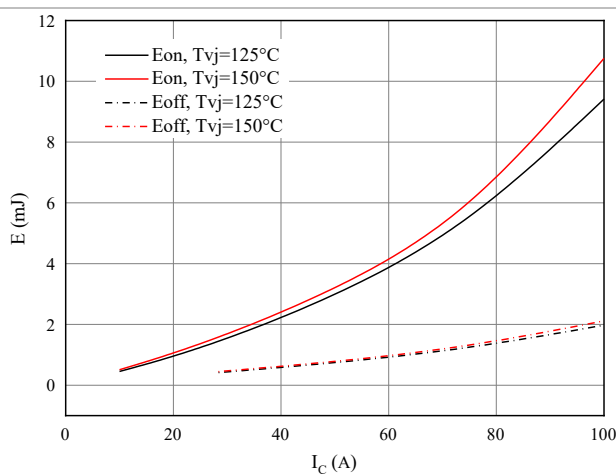
Figure 5. Switching losses of IGBT
