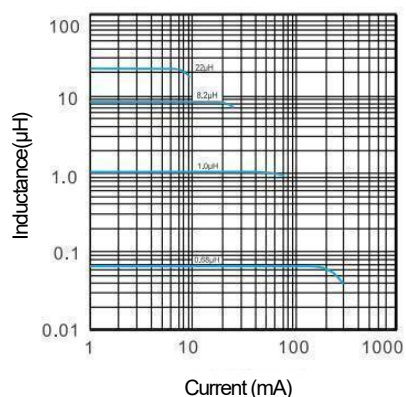
Inductance vs. Current Characteristics
