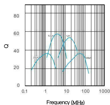
Q vs. Frequency Characteristics
