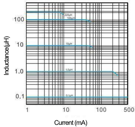
Inductance vs. Current Characteristics
