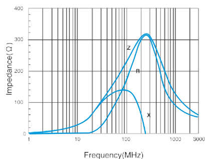
SKCB3216-221
