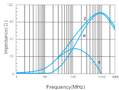
SKCB1608-600
