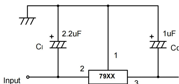
Fig.1 Negative fixed output regulator
