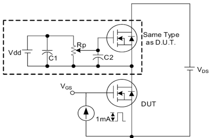
Fig. 3.1 Gate Charge Test Circuit
