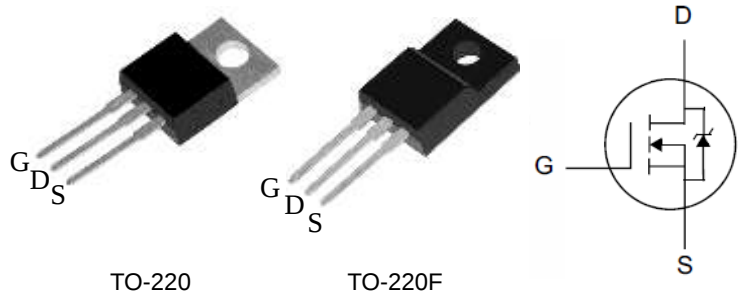
TO-220
