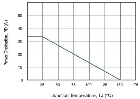
Fig.12 Power Dissipation vs. Junction Temperature
