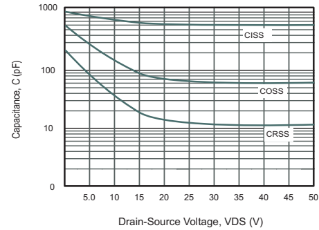
Fig.4 Capacitance Characteristics
