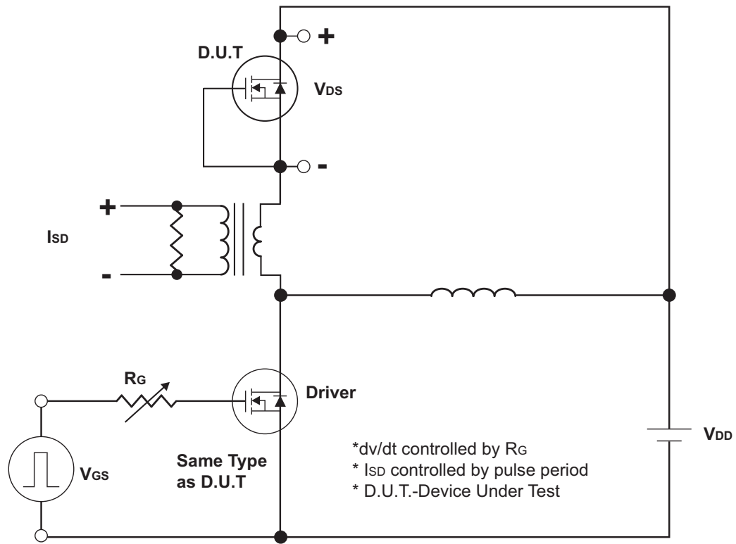
Peak Diode Recovery dv/dt Test Circuit
