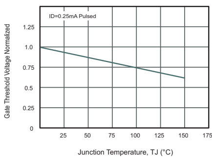
Fig.7 Gate Threshold Voltage vs. Junction Temperature
