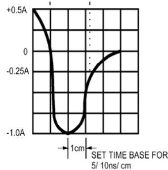
FIG.4- TYPICAL FORWARD CHARACTERISTICS
