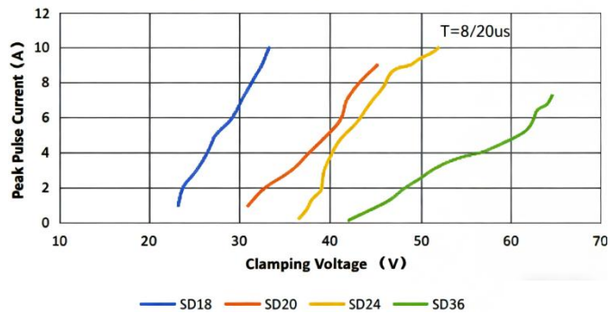
Fig6 Clamping Voltage vs Peak Pulse Current
