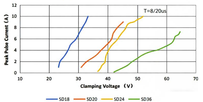
Fig6 Clamping Voltage vs Peak Pulse Current
