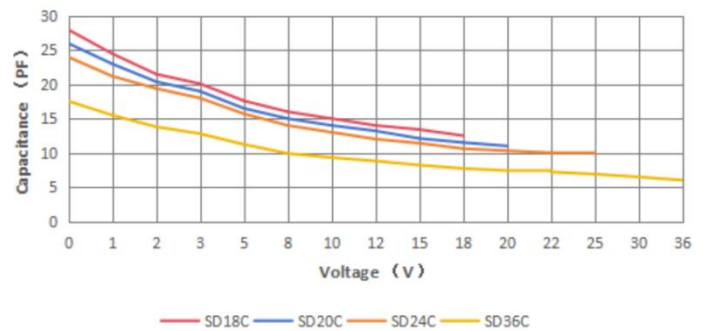
Fig4 Voltage vs Capacitance
