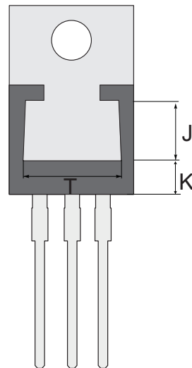
TO-220 mechanical data
