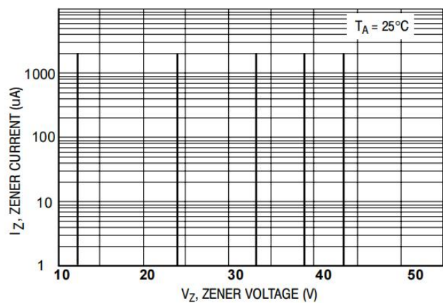
Figure 10. Zener Voltage versus Zener Current (12 to 43 V)
