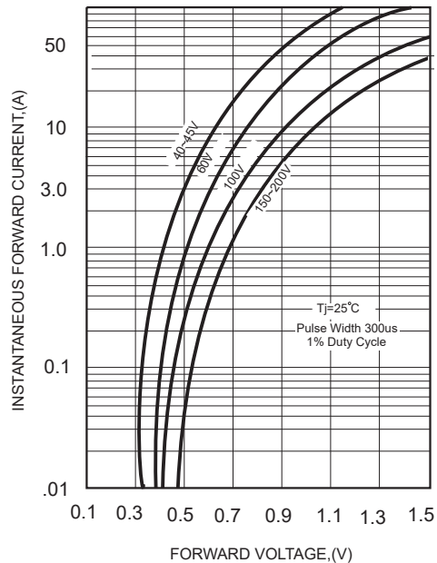
FIG.2-TYPICAL FORWARD CHARACTERISTICS
