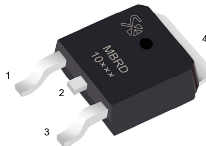
TO-252(D-PAK)
