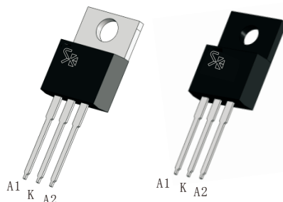
TO-220
