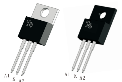
TO-220
