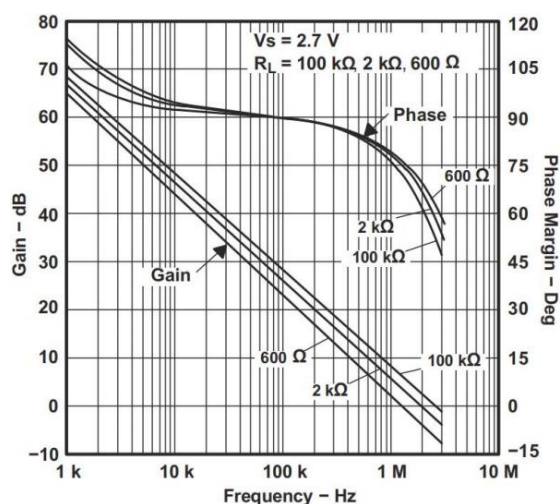
Fig 7. Frequency Response vs. Resistive Load(V CC =2.7V)
