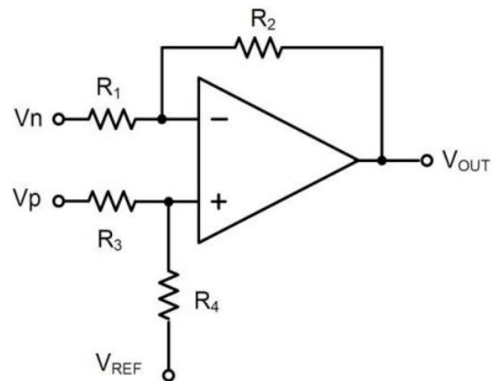
Figure 4. Differential Amplifier
