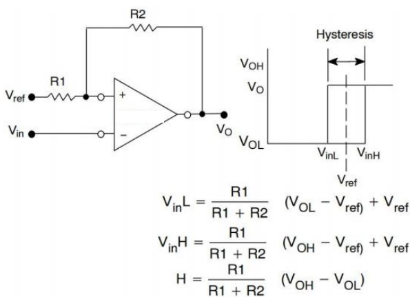
Figure 3. Hysteresis Comparator
