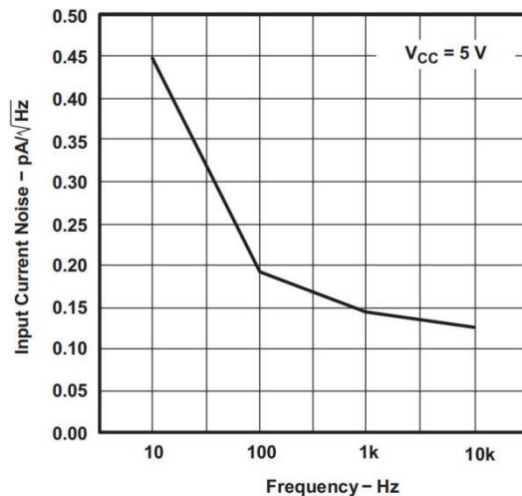
Fig 6. Input Current Noise vs. Frequency(V CC =5V)
