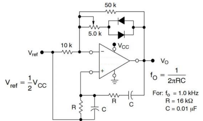
Figure 2. Wien Bridge Oscillator
