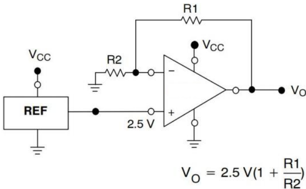
Figure 1. Reference Voltage
