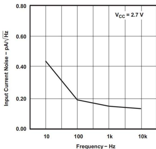
Fig 5. Input Current Noise vs. Frequency(V CC =2.7V)
