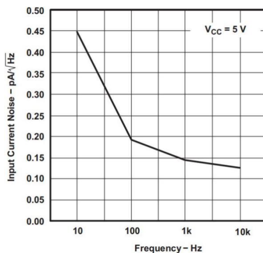
Fig 6. Input Current Noise vs. Frequency( V_{CC}=5\text{V} )
