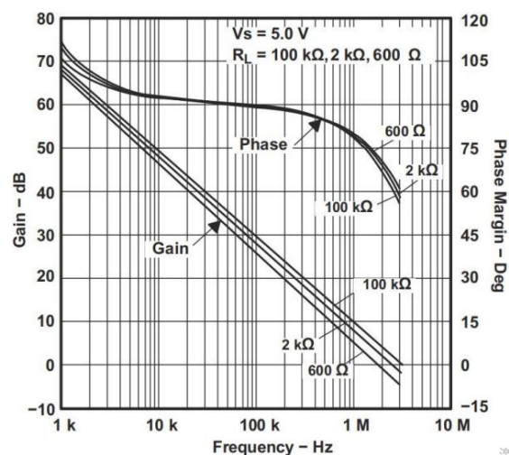
Fig 8. Frequency Response vs. Resistive Load( V_{CC}=5\text{V} )
