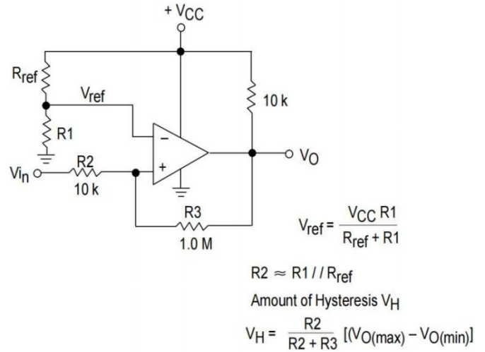
Figure 2. Non-Inverting Comparator with Hysteresis
