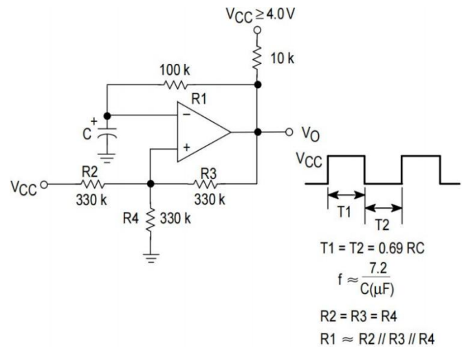
Figure 4. Square Wave Oscillator
