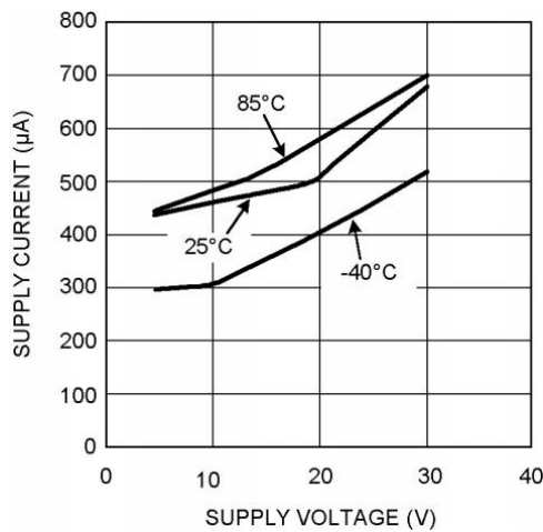
Fig.9 Supply Current vs. Supply Voltage
