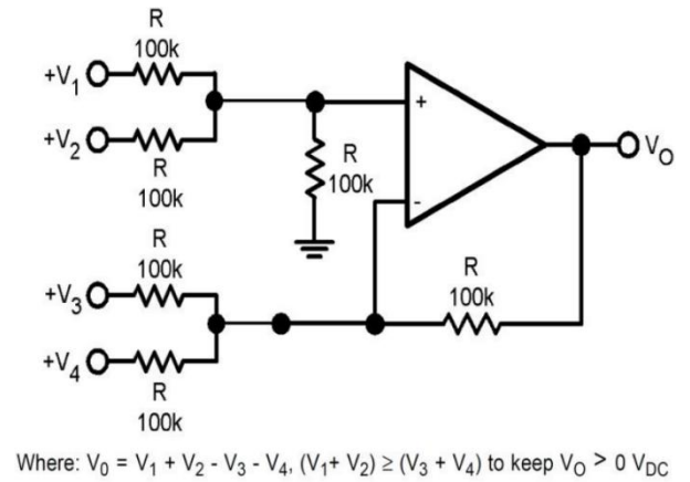
Fig.2 DC Adder Amplifier( V_{IN} \geq 0 V_{DC} ), V_O \geq V_{DC}
