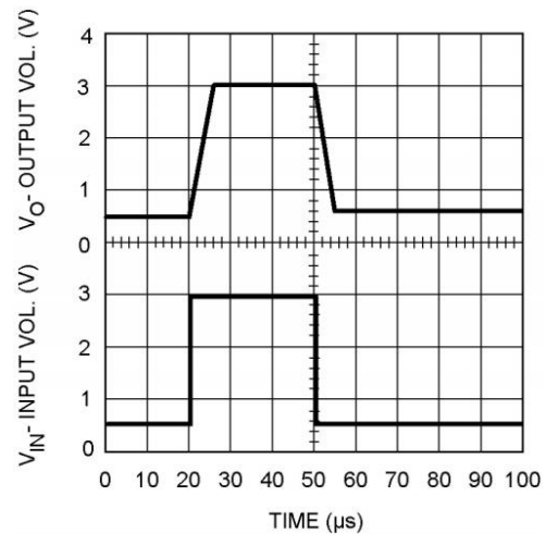
Fig.8 Large signal pulse response
