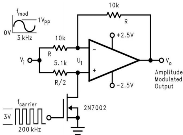
Fig.1 Amplitude Modulator Circuit
