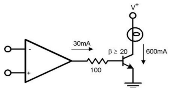
Fig.4 LED Driver
