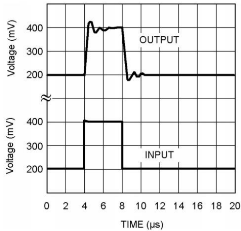
Fig.7 Small signal pulse response
