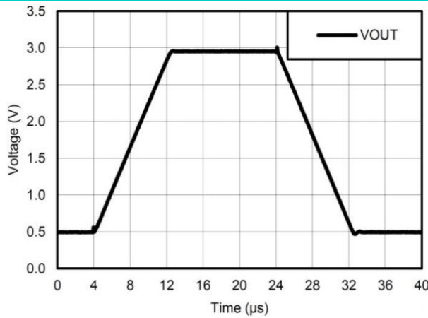
Figure 7: Voltage Follower Large-Signal Response (50pF)
