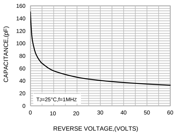
FIG.3-TYPICAL JUNCTION CAPACITANCE
