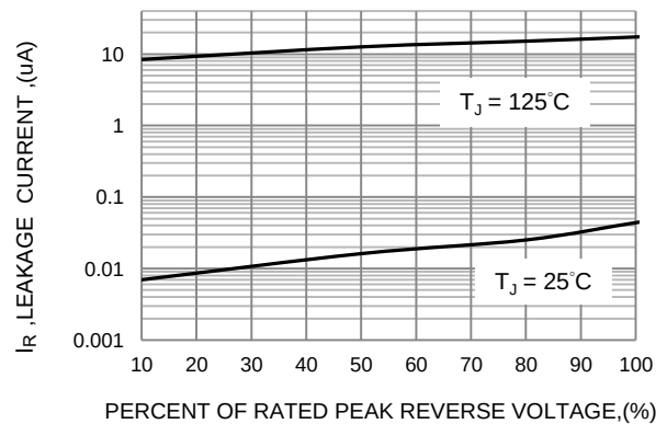
FIG.5-TYPICAL REVERSE CHARACTERISTICS
