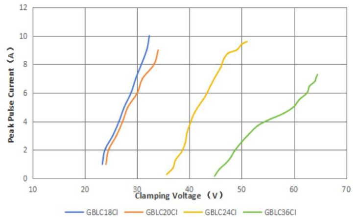
Fig4 Clamping Voltage vs Peak Pulse Current
