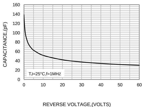
FIG.3-TYPICAL JUNCTION CAPACITANCE
