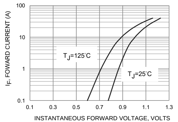
FIG.4-TYPICAL FORWARD CHARACTERISTICS
