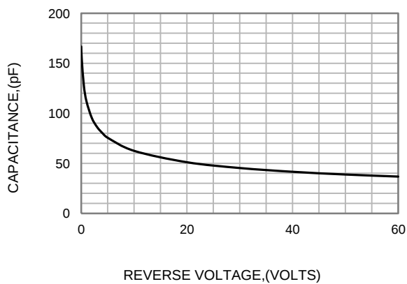
FIG.3-TYPICAL JUNCTION CAPACITANCE
