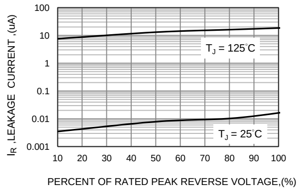
FIG.5-TYPICAL REVERSE CHARACTERISTICS
