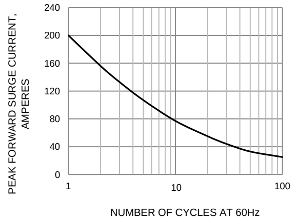
FIG.2-MAXIMUM FOWARD SURGE CURRENT
