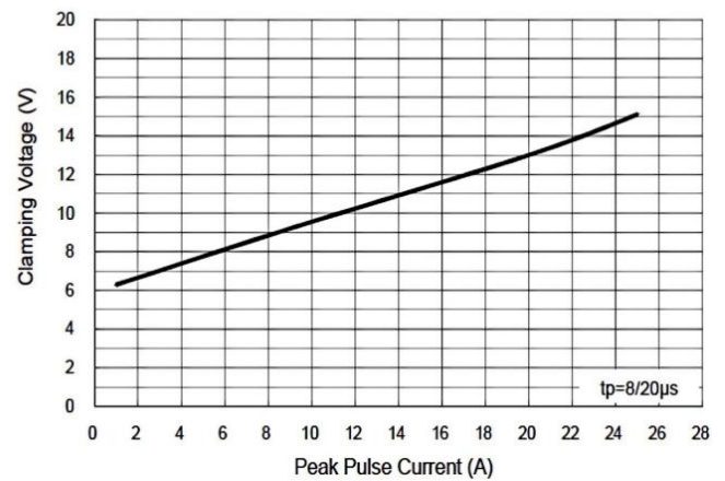
Fig 4 Peak Pulse Current vs Clamping Voltage
