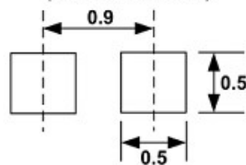
Soldering Footprint
