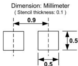
Soldering Footprint
