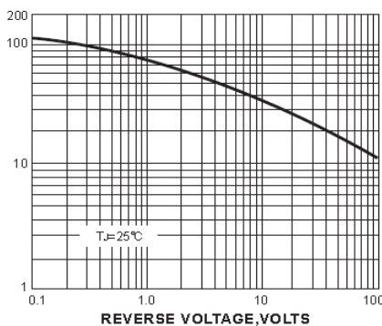
FIG. 5-TYPICAL JUNCTION CAPACITANCE
