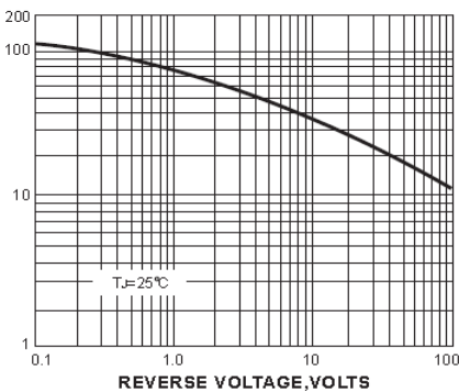
FIG. 5-TYPICAL JUNCTION CAPACITANCE
