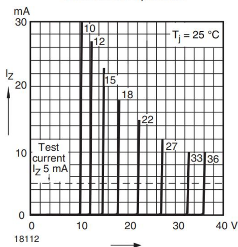
Fig. 4 - Breakdown Characteristics
