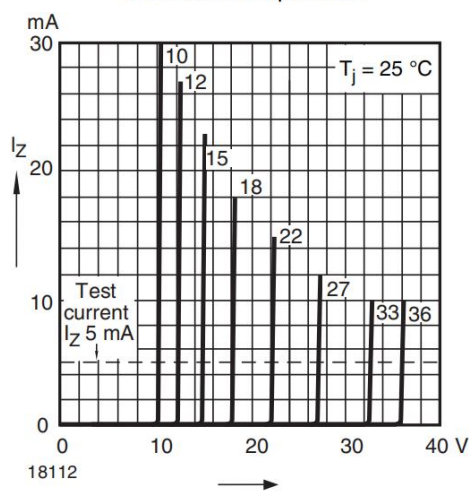
Fig. 4 - Breakdown Characteristics
