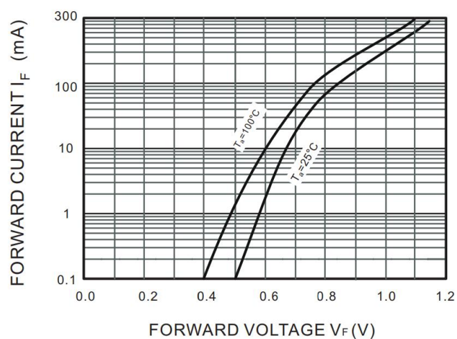
Fig.3 Forward Characteristics
