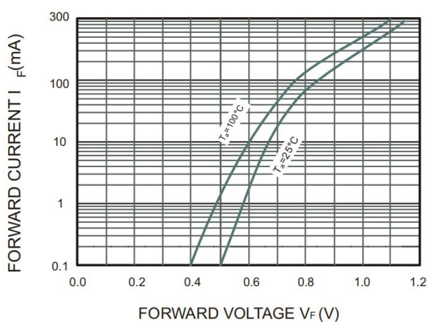
Fig.3 Forward Characteristics
