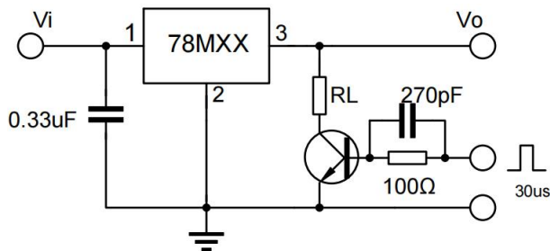
Fig.2 LOAD REGULATION
